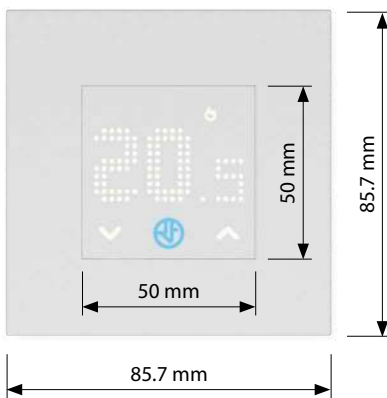
Mounting in 2 module or 65 mm round wall boxes
