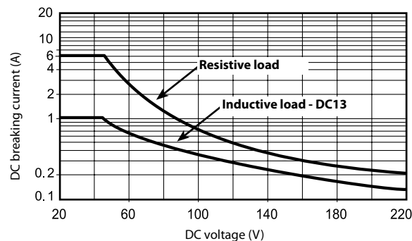
H 7S12* - Maximum DC breaking capacity - 7S.12
