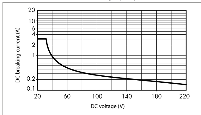
H 7S16/36 - Maximum DC13 breaking capacity - 7S.16/36
