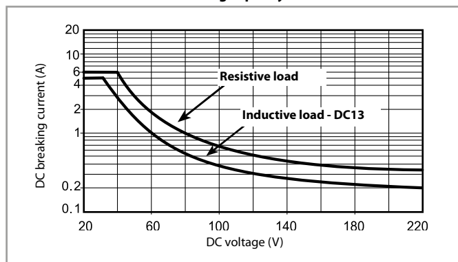
H 7S43* - Maximum DC breaking capacity - 7S.43/63
