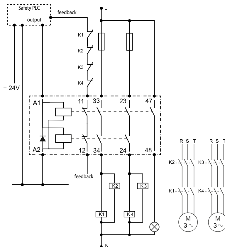
Type 75.43/63
