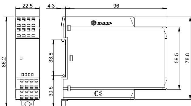
Type 75.32 Box clamp
