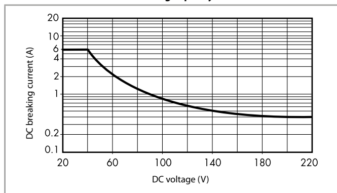
H 7S16* - Maximum DC1 breaking capacity - 7S.16/36
