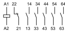
7S.16/36...5510
