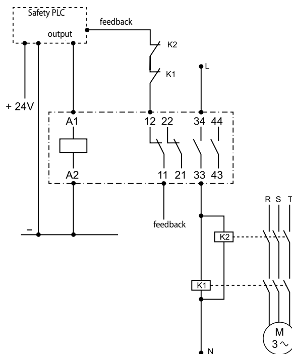
Type 75.x4...4220
