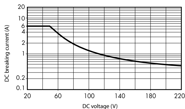
H 7S14* - Maximum DC1 breaking capacity - 7S.14/34
