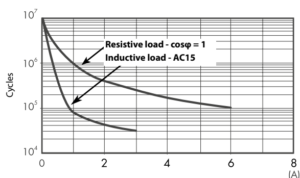
F 7S14 - Electrical life (AC) v contact current - 7S.14/34
