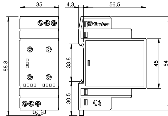
Type 70.42 Box clamp
