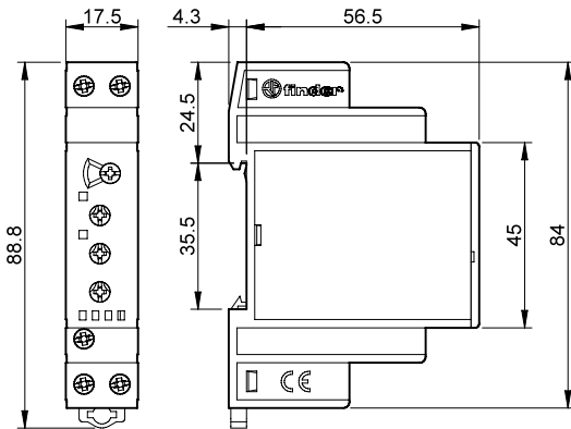
Type 70.41 Box clamp
