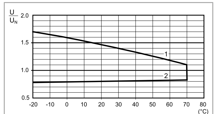
R 66 - AC coil operating range v ambient temperature
