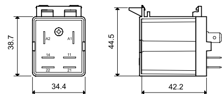
065.08 with relay
