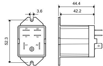
065.05 with relay
