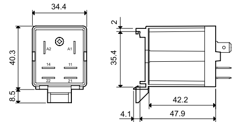
065.07 with relay
