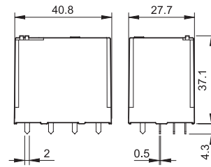
Type 56.44
