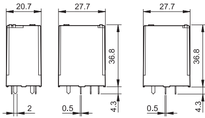
Types 56.42/42-0300
