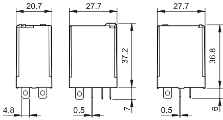
Types 56.32/32-0300
