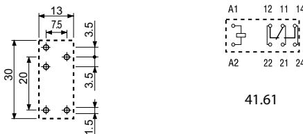
95.13.2 Copper side view
