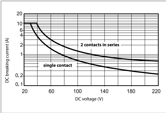
H 40.6 - Maximum DC1 breaking capacity Type 40.62
