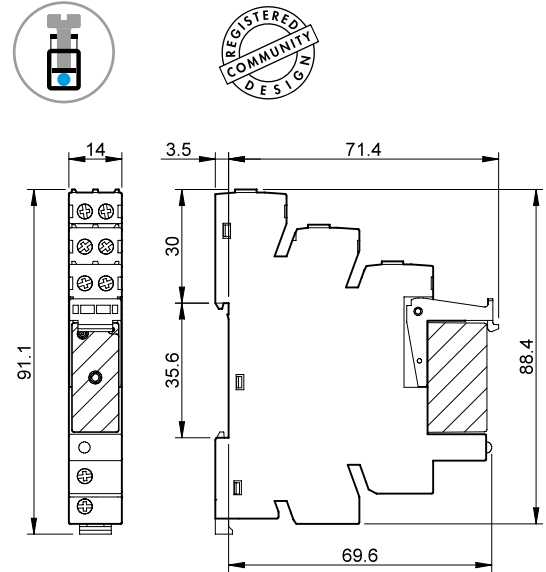
Types 38.01 38.31 38.52 Box clamp
