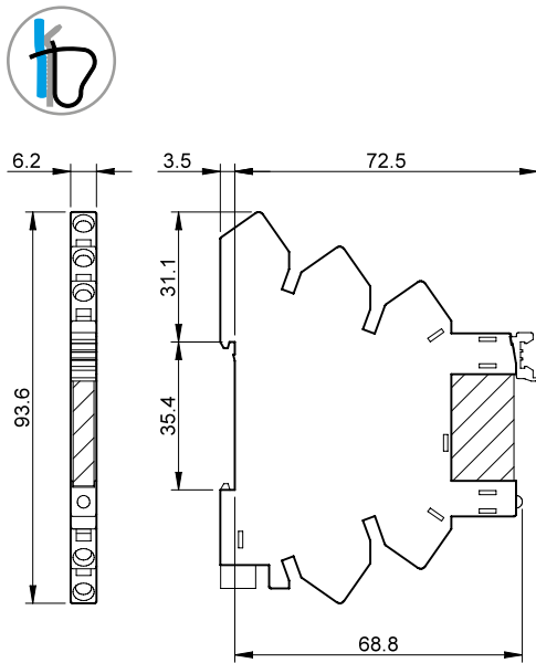
Types 38.61 / 38.61.3 38.91 / 38.91.3 Screwless terminal
