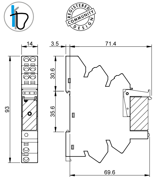
Types 38.11 38.41 38.62 Screwless terminal
