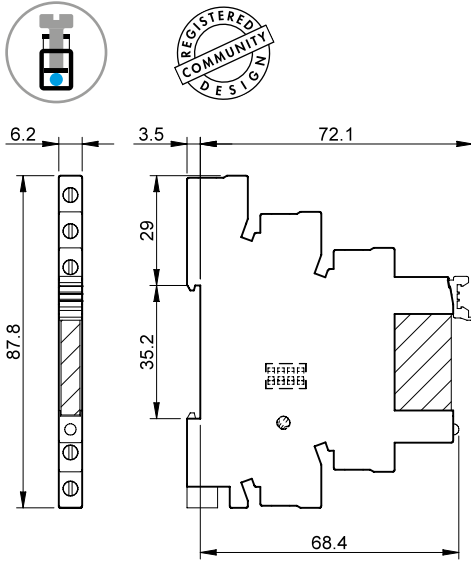
Types 38.21 38.51 / 38.51.3 38.81 / 38.81.3 Box clamp
