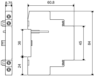
Types 022.73/022.75 Box clamp
