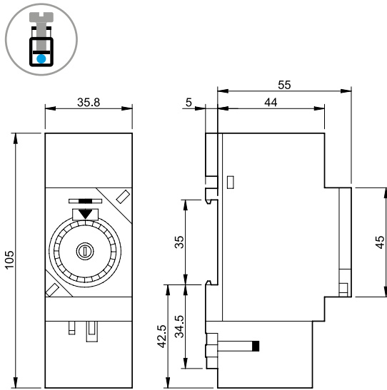
Type 12.31 Box clamp
