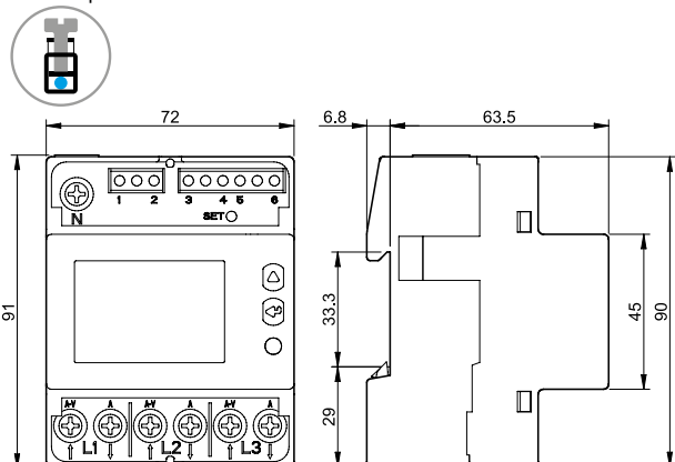
Type 7E.78.8.400.0112 Box clamp
