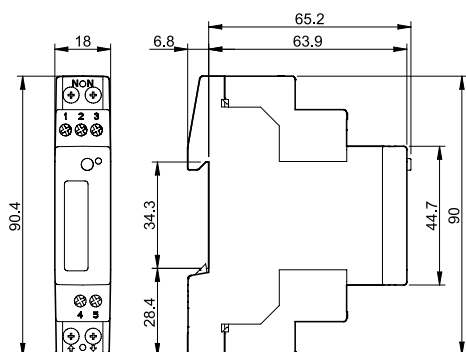
Type 7E.78.8.400.0212 Box clamp
