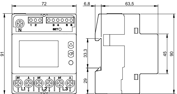
Type 7E.78.8.400.0410 Box clamp
