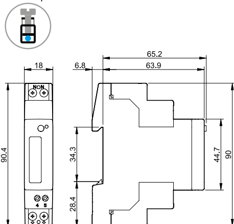
Type 7E.78.8.400.0112 Box clamp
