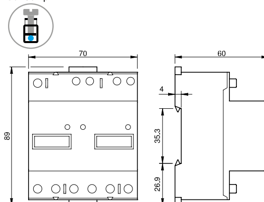
Type 7E.64.8.230.0010 Box clamp
