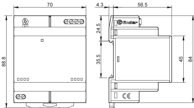
Type 78.1B Box clamp
