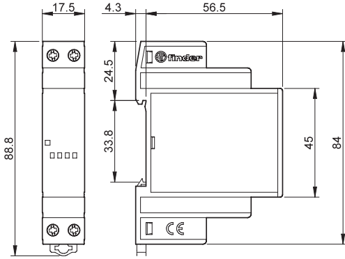
Types 78.36/78.50/78.60 Box clamp
