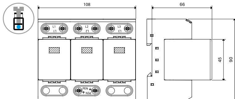
Type 7P.03 Box clamp
