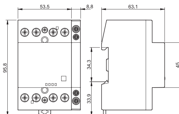
Tipo 22.44/22.64 + 022.63/022.65 Morsetti a vite
