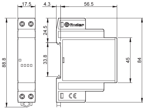
Type 78.36/78.50/78.60 Kooiklemmen
