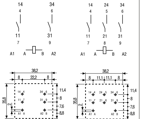
62.22 - 4300 Copper side view
