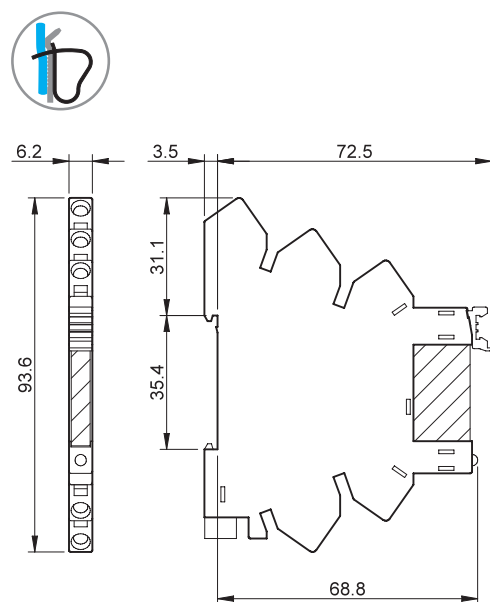
Tipi 38.61 / 38.61.3 38.91 / 38.91.3 Morsetti a molla
