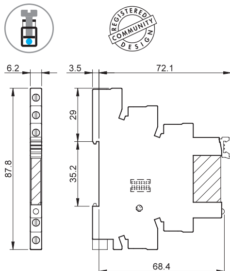
Tipi 38.21 38.51 / 38.51.3 38.81 / 38.81.3 Morsetti a bussola
